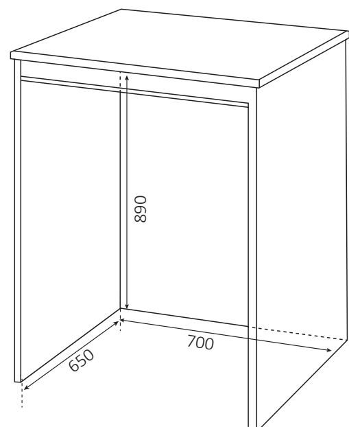
Misure interne del mobile Internal dimensions
